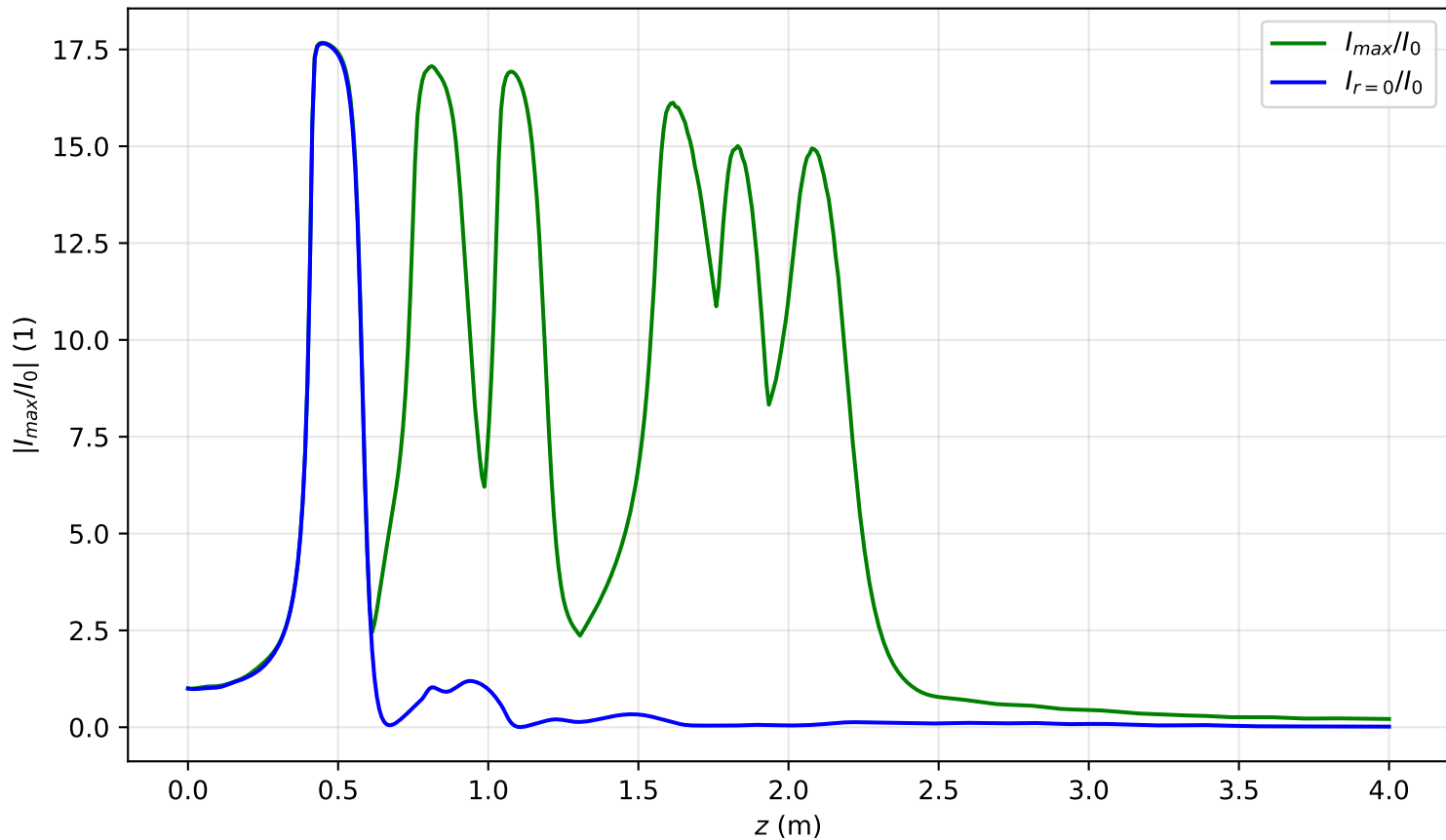
I_{max}(x = 0, y = 0, z)/I_0 , Pin=6.3Pcr, noisy input, artificial time
